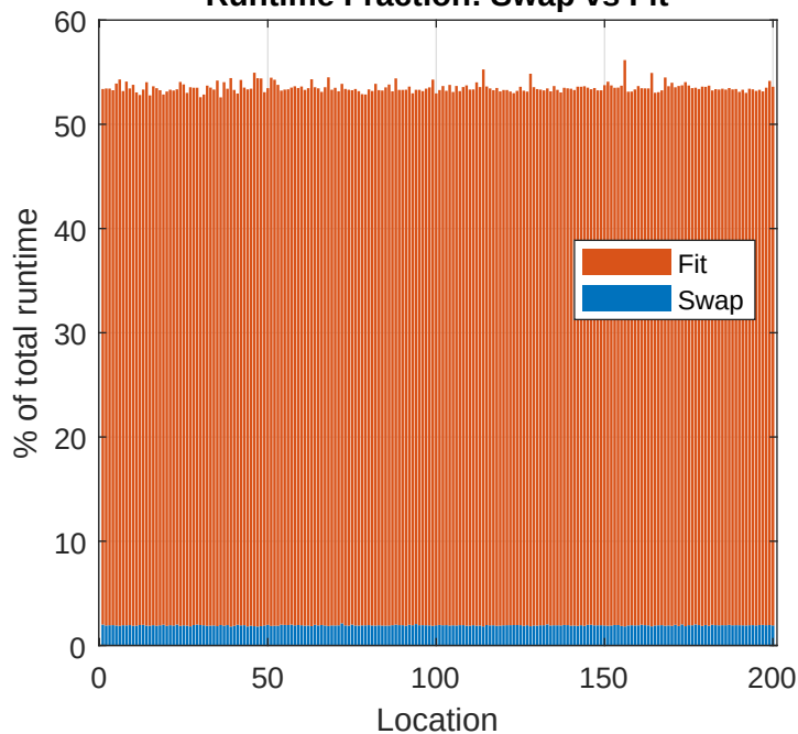
Runtime Fraction: Swap vs Fit 2D Polynomial
